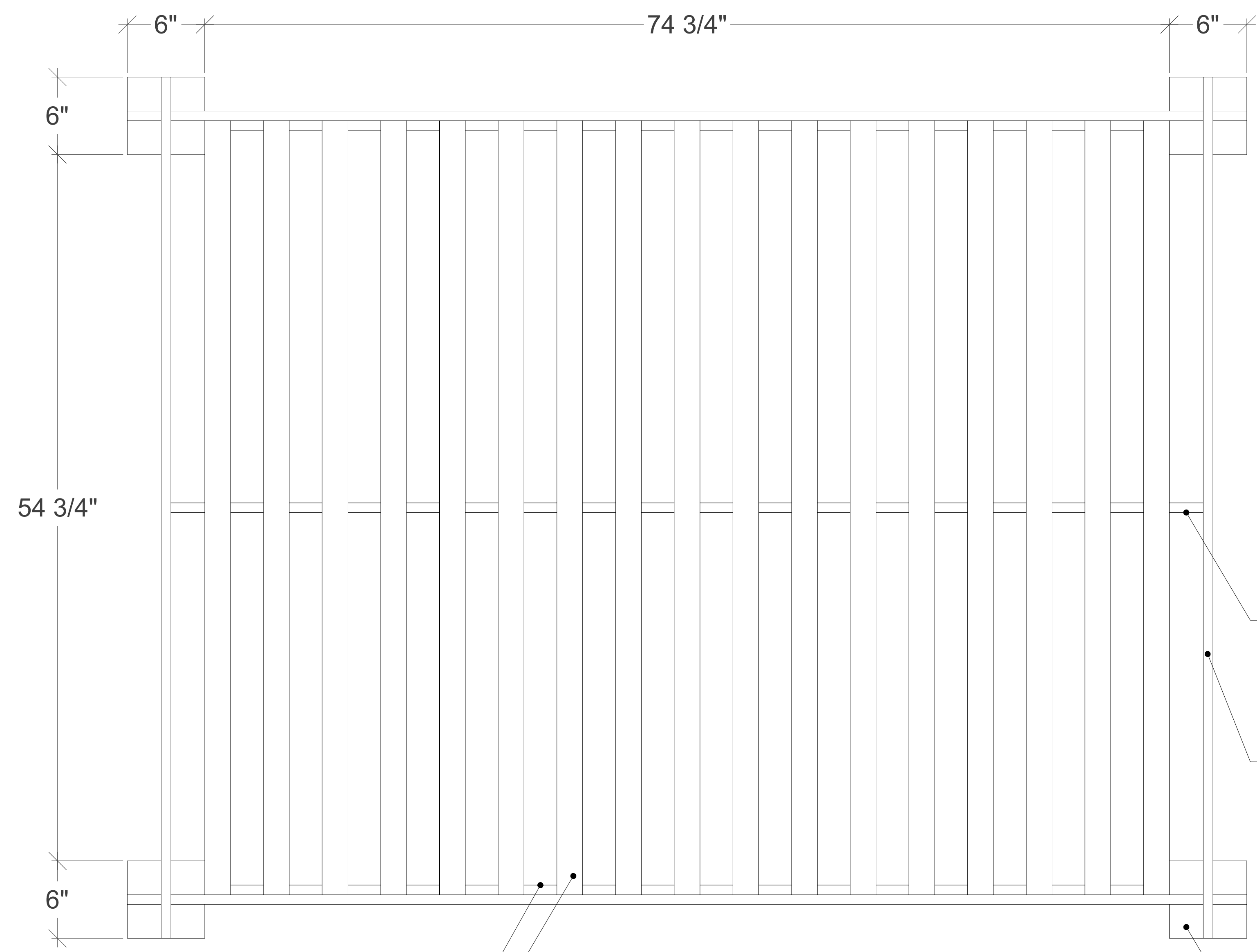
Top view
