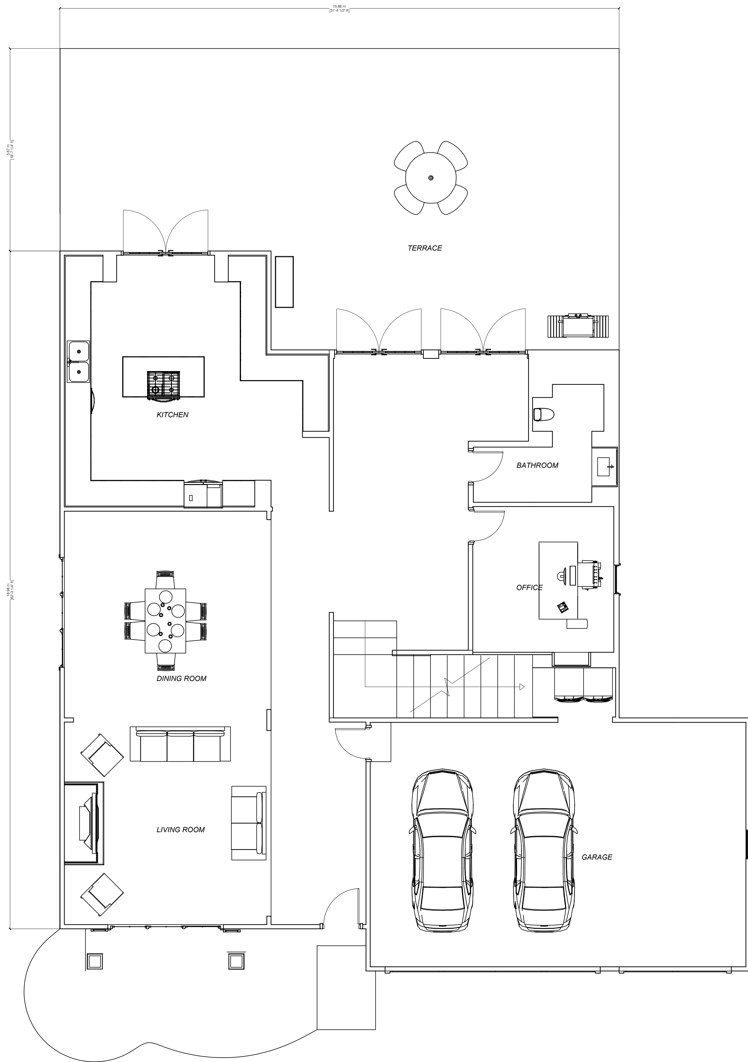
First Floor Architectural Plan
