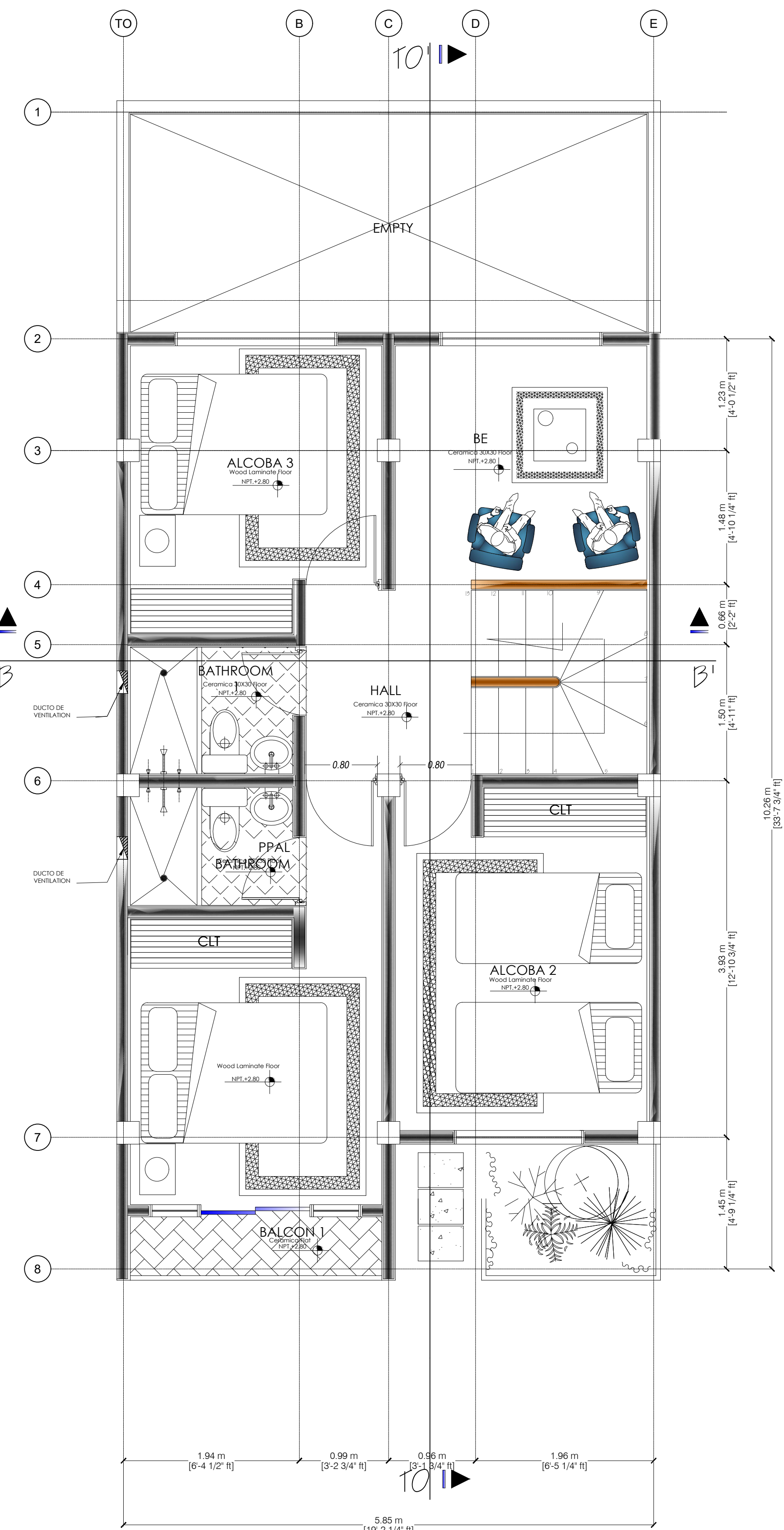
SECOND FLOOR FLOOR
